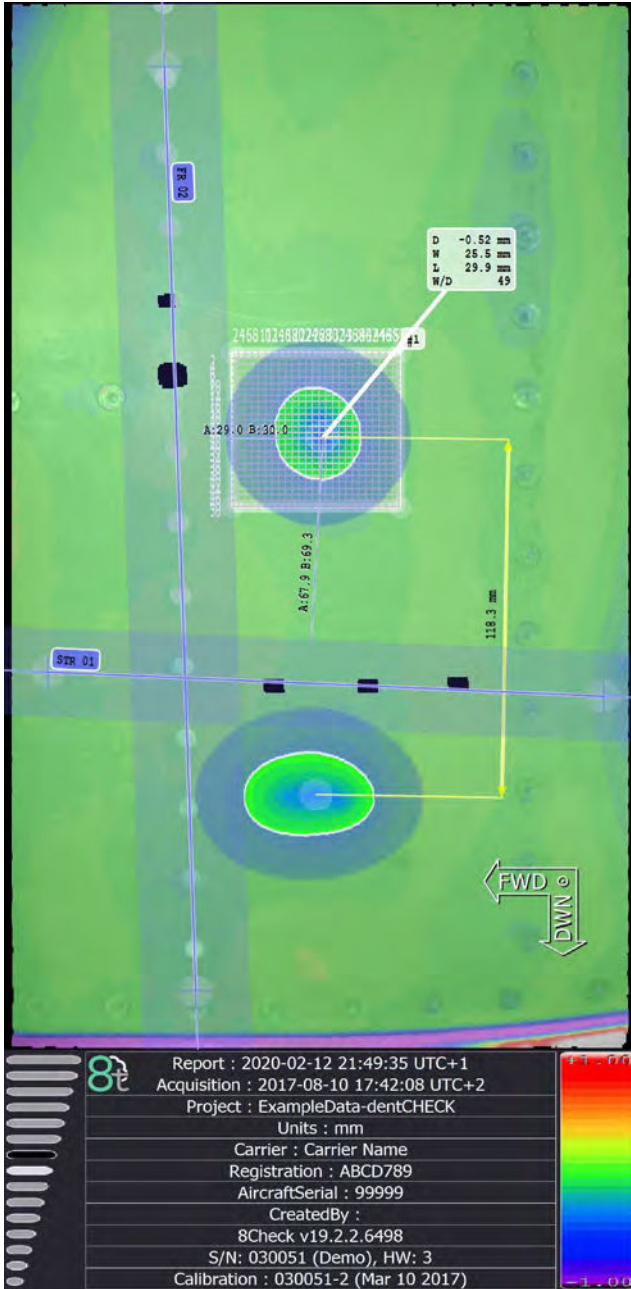
3D Dent Map of Inspected Area
