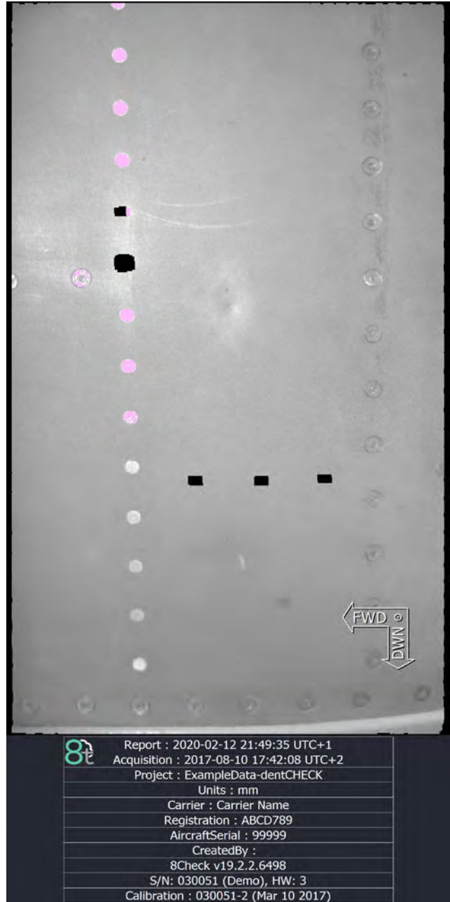
2D Photo of Inspected Area (simultaneously captured)
